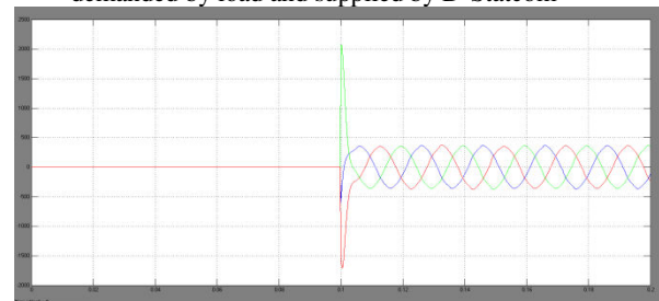
Fig. 12 shows the D-STATCOM injected harmonic current
