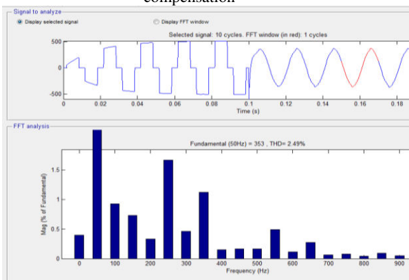
Fig.14 shows the THD response of source current after compensation
