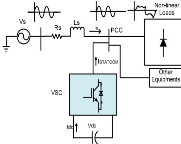
Figure 3: Power system with D-STATCOM
