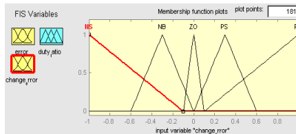
Fig. 8. The Membership Function plots of change error
