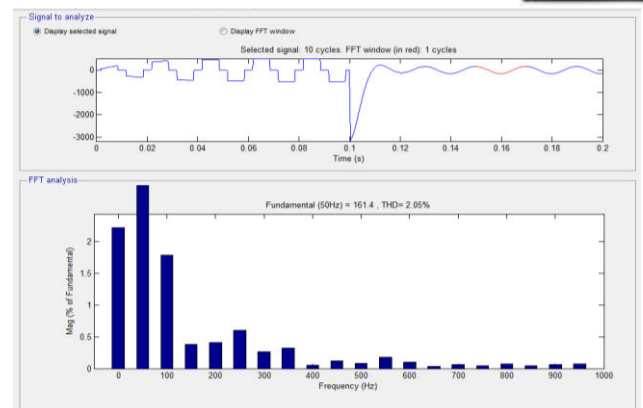
Fig.17 shows the THD response of source current after compensation with fuzzy logic controller
