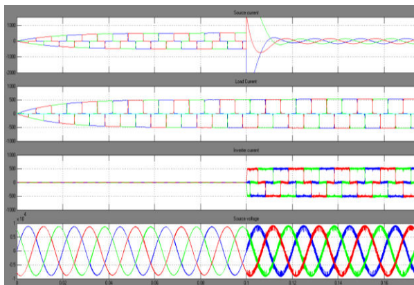
Fig.16 shows the simulation waveforms of source current, load current, injected current and source voltage with fuzzy logic controller
