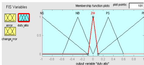
Fig. 9. the Membership Function plots of duty ratio
