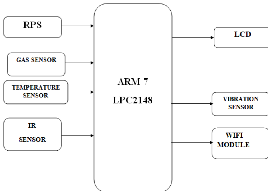
4 Fig.6.1. Block diagram
