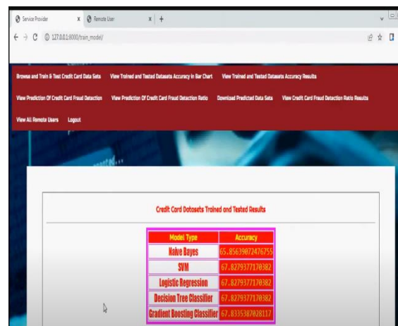
Fig.7. Algorithms applied.
