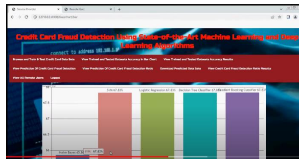
Fig.8. Prediction Graphs.
