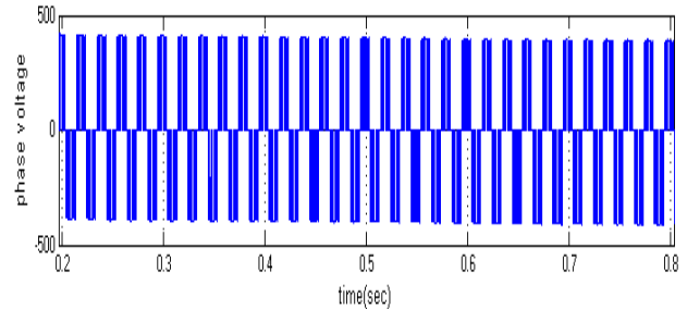
Fig.27. Simulated wave form of Phase voltage of the Inverter at MI=1 with Switch open fault.
