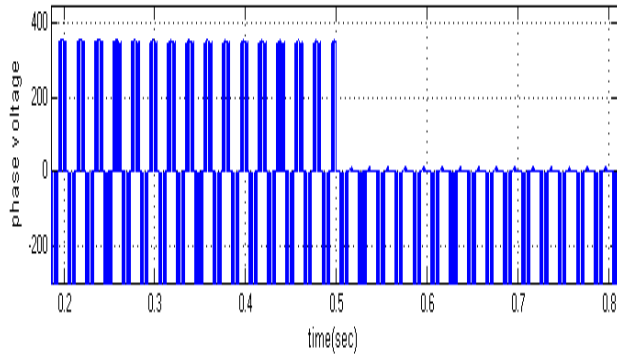
Fig.23. Simulated wave form of Phase voltage of the Inverter at MI=1 with Gate short fault.
