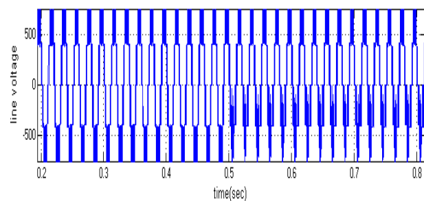
Fig.25. Simulated wave form of Line Voltage of the Inverter at MI=1 with Switch open fault.
