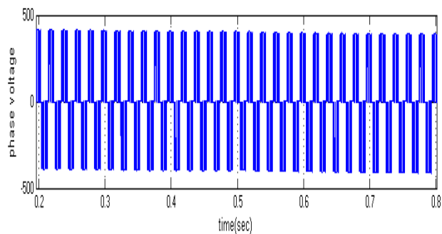
Fig. 19. Simulated wave form of Phase voltage of the Inverter at MI=1 with Gate open fault.
