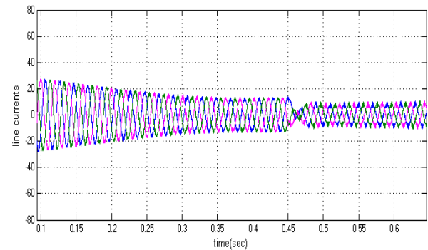
Fig.35. Simulated wave form of Line Current of the Inverter at MI=1 with Switch open fault.
