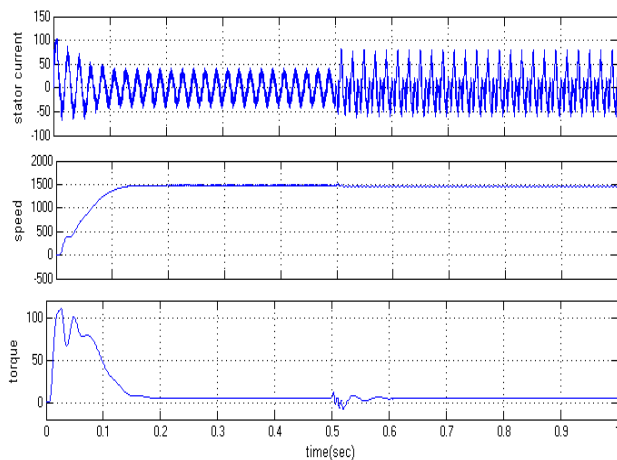
Fig.24. Performance characteristics of Current, Speed and Torque at MI=1 with Gate short fault.
