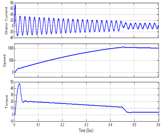
Fig.41. Performance characteristics of Current, Speed and Torque at MI=1 with Switch Short fault.
