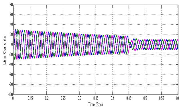
Fig.39. Simulated wave form of Line Current of the Inverter at MI=1 with Switch Short fault.
