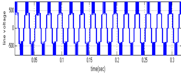
Fig.9. Simulated wave form of Line Voltage of the Inverter at MI=1 with Diode open fault
