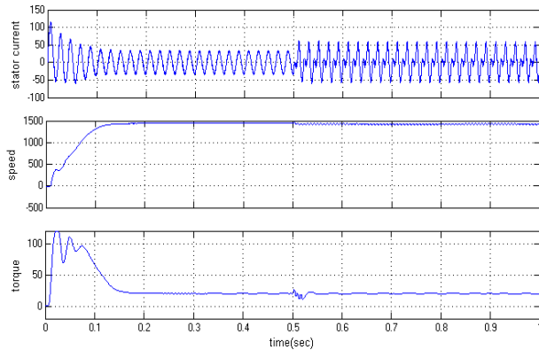
Fig.32. Performance characteristics of Current, Speed and Torque at MI=1 with Switch short fault.
