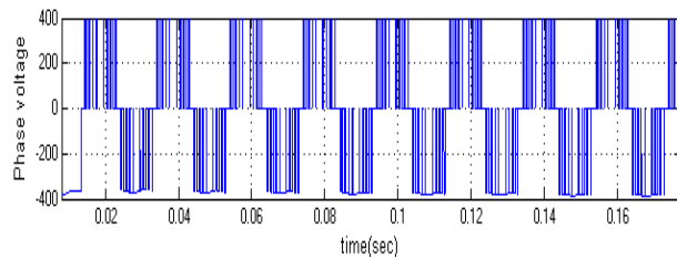
Fig.11. Simulated wave form of Phase voltage of the Inverter at MI=1 with Diode open fault.
