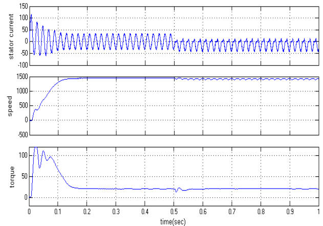
Fig.28. Performance characteristics of Current, Speed and Torque at MI=1 with Switch open fault.
