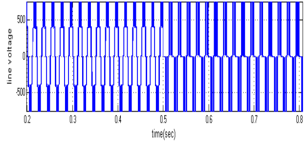
Fig.13. Simulated wave form of Line Voltage of the Inverter at MI=1 with Diode short fault.
