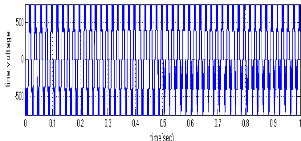
Fig. 17. Simulated wave form of Line Voltage of the Inverter at MI=1 with Gate open fault.
