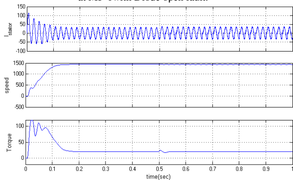
Fig.12. Performance characteristics of Current, Speed and Torque at MI=1 with Diode open fault.
