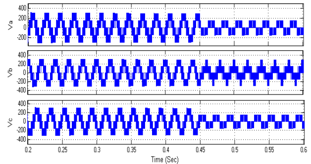
Fig.34. Simulated wave form of Line Voltage of the Inverter at MI=1 with Switch open fault.
