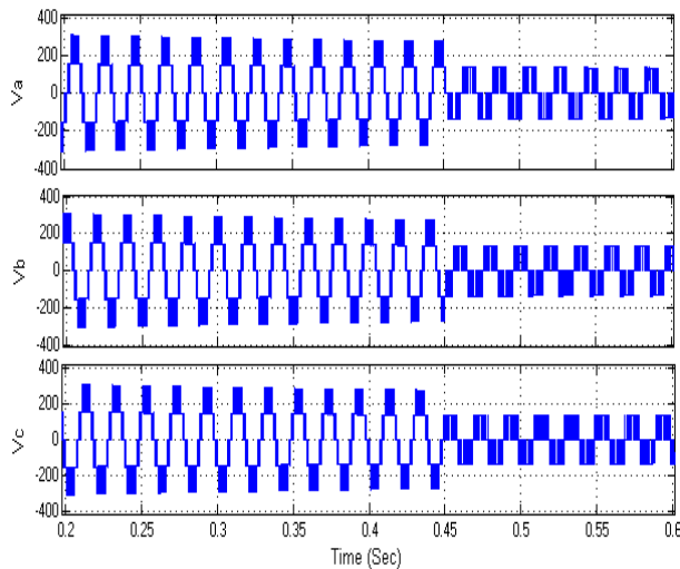
Fig.38. Simulated wave form of Line Voltage of the Inverter at MI=1 with Switch Short fault.
