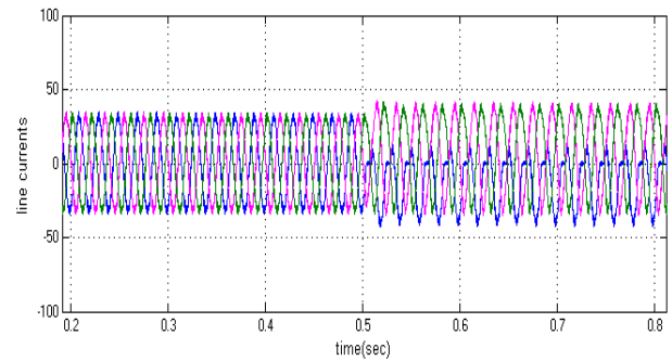
Fig.26. Simulated wave form of Line Current of the Inverter at MI=1 with Switch open fault.
