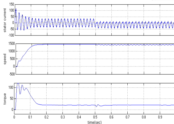
Fig. 20. Performance characteristics of Current, Speed and Torque at MI=1 with Gate open fault.
