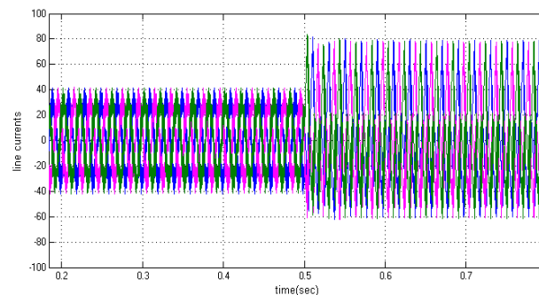
Fig. 22. Simulated wave form of Line Current of the Inverter at MI=1 with Gate short fault.
