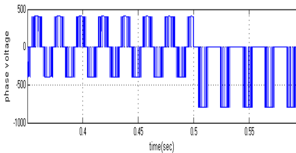
Fig.31. Simulated wave form of Phase voltage of the Inverter at MI=1 with Switch short fault.
