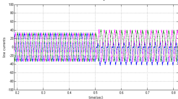
Fig. 18. Simulated wave form of Line Current of the Inverter at MI=1 with Gate open fault.
