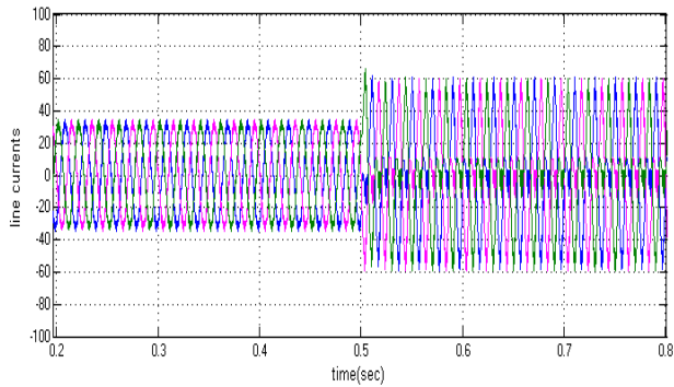
Fig.30. Simulated wave form of Line Current of the Inverter at MI=1 with Switch short fault.
