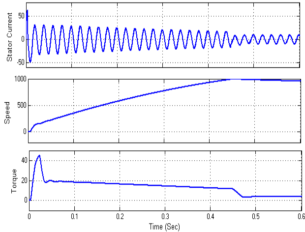
Fig.37. Performance characteristics of Current, Speed and Torque at MI=1 with Switch open fault.
