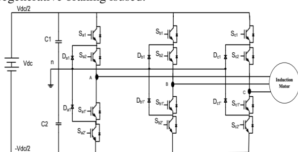
Fig.1. Neutral Point Clamped three level Inverter based Induction motor drive.
