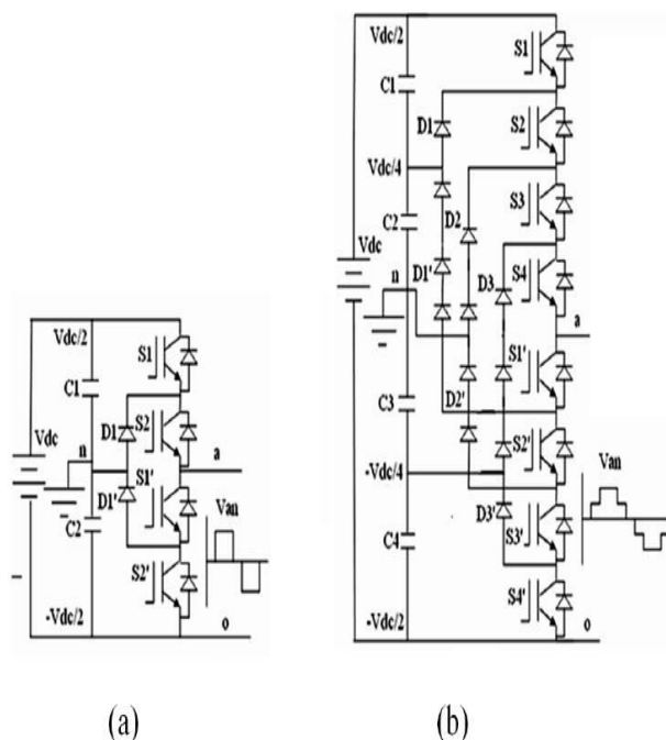
Fig.7 Topology of the diode-clamped inverter (a) three-level inverter, (b) five-level inverter
