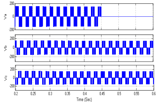
Fig.36. Simulated wave form of Phase voltage of the Inverter at MI=1 with Switch open fault.
