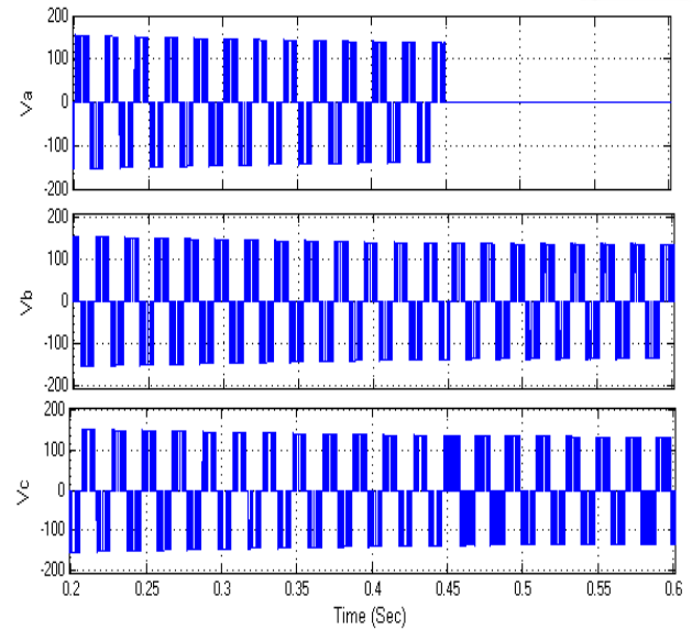
Fig.40. Simulated wave form of Phase voltage of the Inverter at MI=1 with Switch Short fault.
