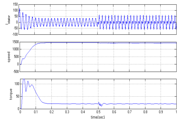
Fig.16. Performance characteristics of Current, Speed and Torque at MI=1 with Diode short fault.
