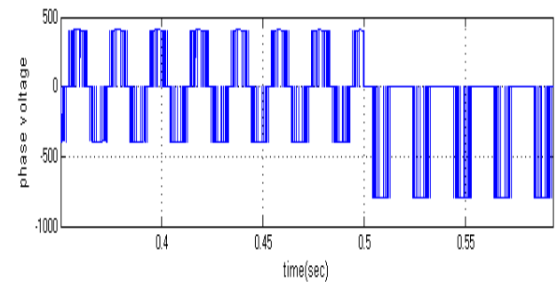
Fig.15. Simulated wave form of Phase voltage of the Inverter at MI=1 with Diode short fault.
