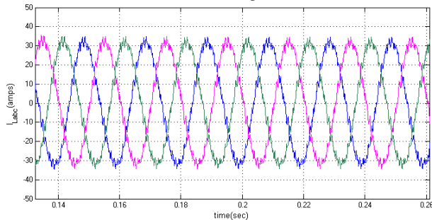
Fig.10. Simulated wave form of Line Current of the Inverter at MI=1 with Diode open fault.
