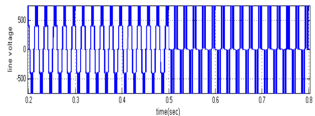
Fig.29. Simulated wave form of Line Voltage of the Inverter at MI=1 with Switch short fault.
