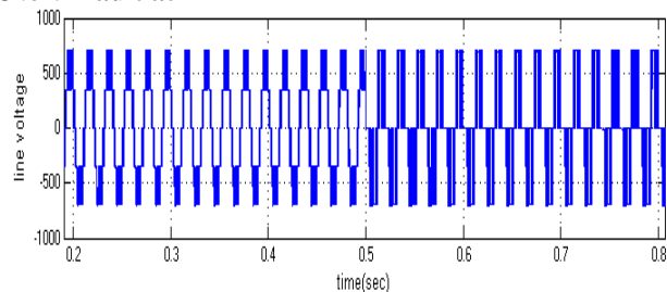
Fig. 21. Simulated wave form of Line Voltage of the Inverter at MI=1 with Gate short fault.
