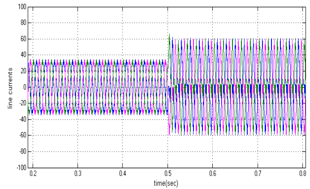
Fig.14. Simulated wave form of Line Current of the Inverter at MI=1 with Diode short fault.
