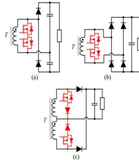
Fig. 5. Derived ABR topologies: (a) voltage-doubler, (b) full-bridge, and (c) center-tapped.
