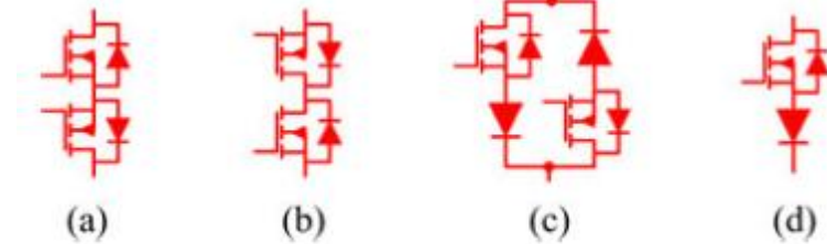
Fig. 4. (a)–(c) Realizations of bidirectional switch and (d) unidirectional switch.
