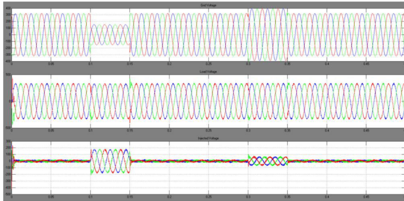
Fig 7. Waveforms for Sag & Swell Condition
