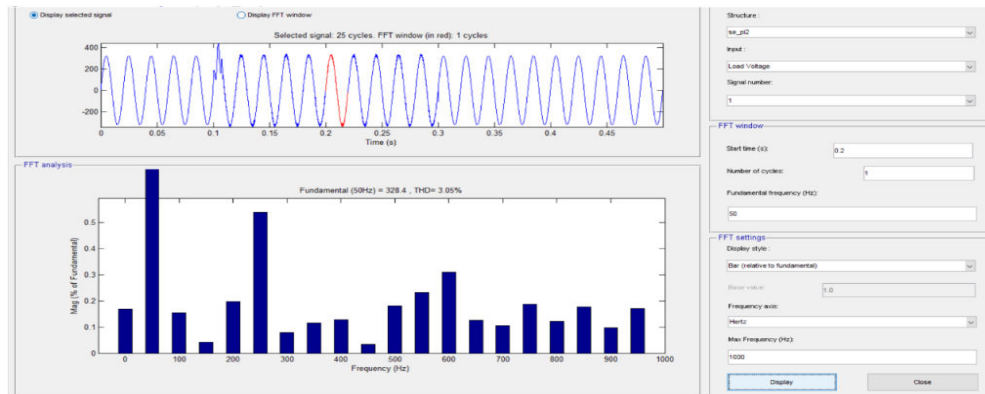
Fig 6. Load Voltage THD
