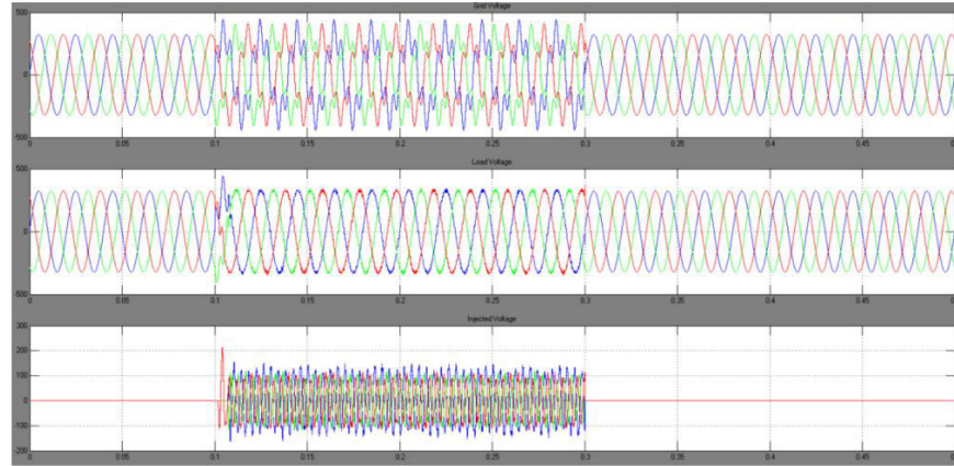
Fig 5. Waveforms for Injection of 5th Harmonic
