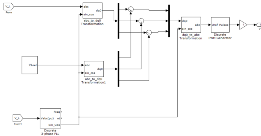
Fig 2. Controller System
