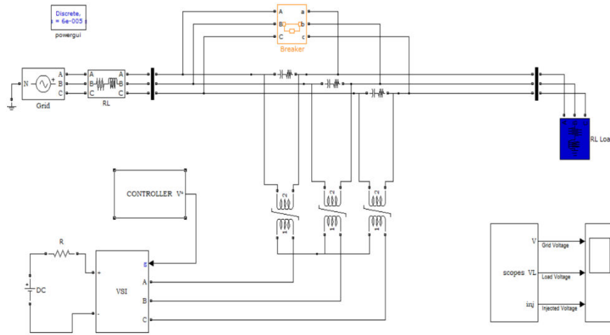
Fig 1. MATLAB/SIMULINK diagram of proposed DVR system
