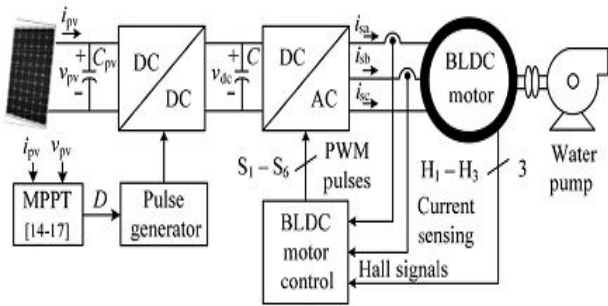
Fig.1. Conventional SPV-fed BLDC motor-driven water pumping system
