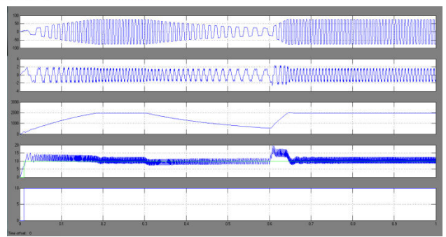
(c) Fig.7 Dynamic performances of the proposed SPV array-based zeta converter-fed BLDC motor drive for water pump. (a) SPV array variables. (b) Zeta converter variables. (c) BLDC motor-pump variables.
