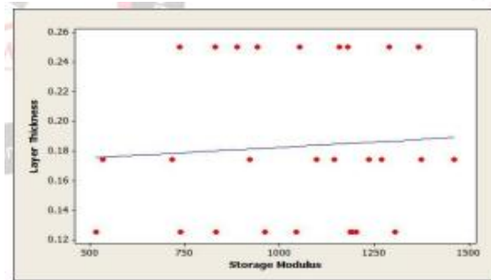
Figure 2 Fitted line plot for Storage Modulus Vs. Layer Thickness(PC)
