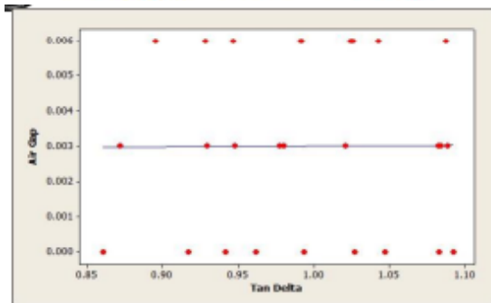
Figure 4 Fitted line plot for Tan Delta Vs. Air Gap (PC)
