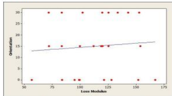
Figure 3 Fitted line plot for Loss Modulus Vs. Orientation (PC)
