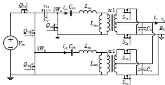
Fig. 1. Two-phase interleaved flying-capacitor LLC (TIFLLC) converter topology.
