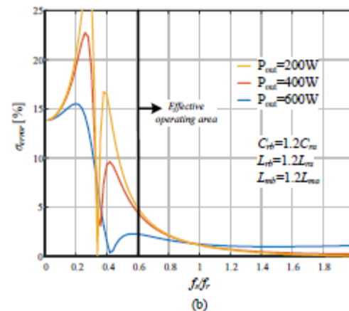
Fig. 8. Current error between the phases as a function of the switching frequency for: (a) C_{rb}=1.2C_{ra} , (b) worst case component's mismatch: C_{rb}=1.2C_{ra} , L_{rb}=1.2L_{ra} , L_{mb}=1.2L_{ma} .
