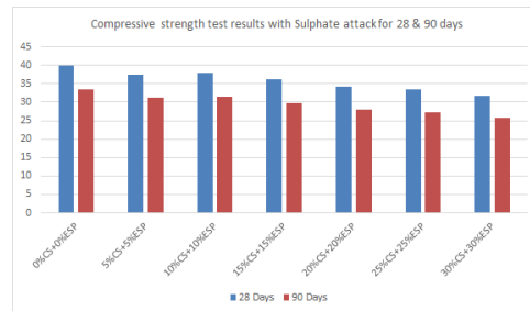
Graph 6.5- Compressive strength test results with Sulphate attack for 28 & 90 days
