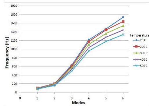
Graph between Modes and Frequency
