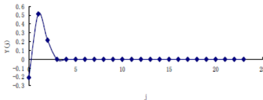
Figure 5. Periodic response factors Y^*(j) curve.
