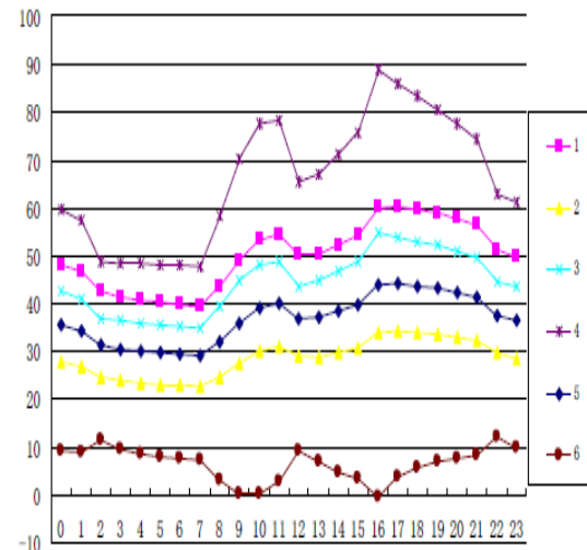
figure3. The hourly value of the air conditioning heating load temperature for six kinds of south wall in winter in Harbin
