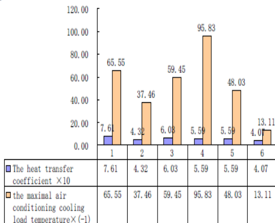
figure1. The heat transfer coefficient data and the maximal air conditioning cooling load temperature value for 6 kinds of south wall in summer in Nanjing
