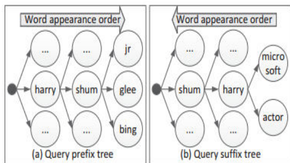
Figure 4: The data structures to index search logs
