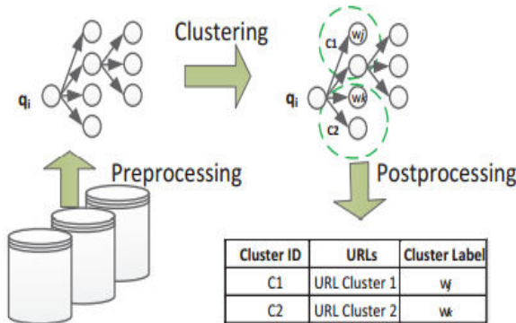
Figure 3: The flow of clustering method
