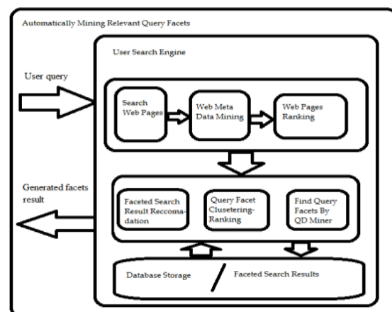
Fig.1: System architecture of automatically Query facet mining
