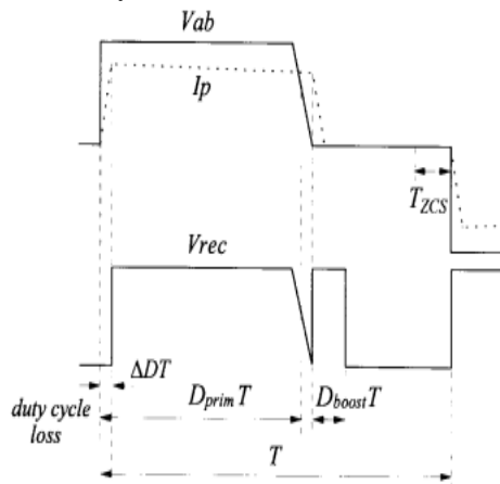
Fig. 5. Primary and secondary rectifier voltage waveforms.
