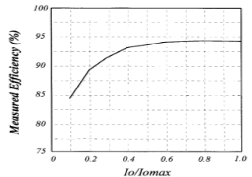
Fig. 14. Measured efficiencies.
