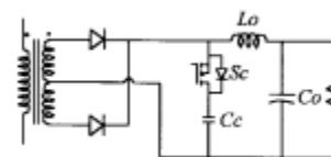
Fig. 7. Circuit diagram of the active clamp circuit for a center-tapped transformer.
