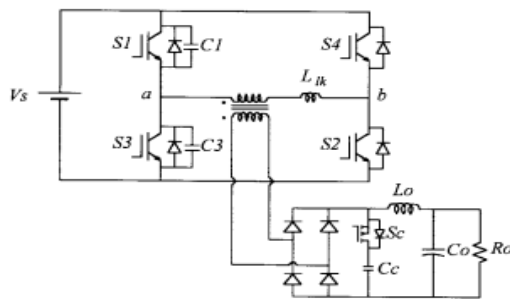
Fig. 1. Circuit topology of the proposed ZVZCS FB PWM converter.
