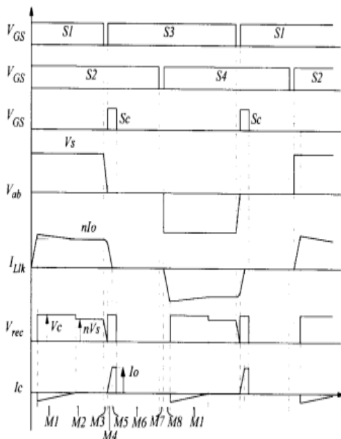
Fig. 3. Operation waveforms.
