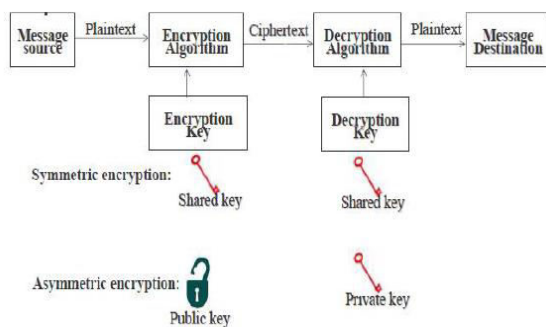
Fig 2: Cryptography
