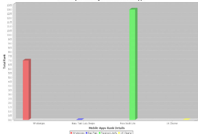
Fig 2:.. RANKING RESULTS
