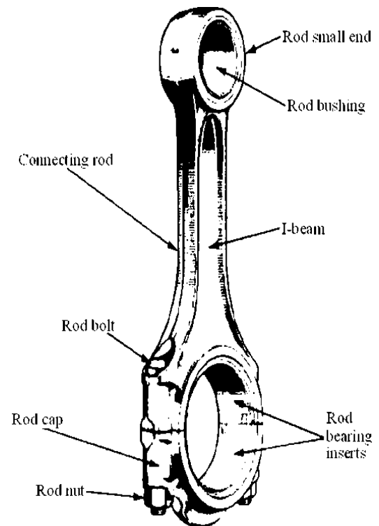
Fig.1 Connecting rod nomenclature
